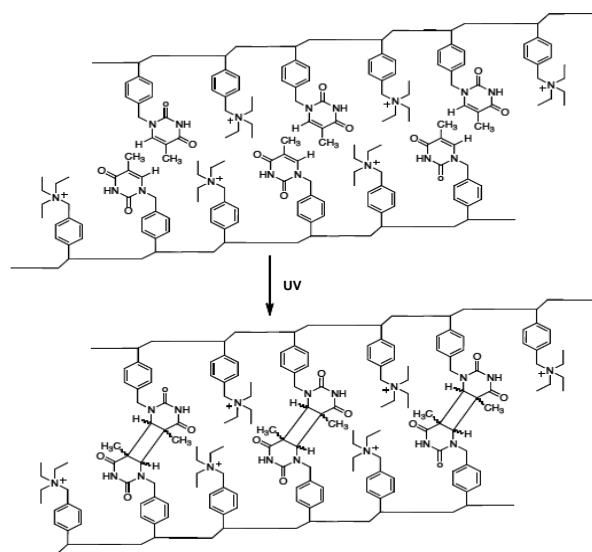
Scheme 1. Photo-dimerization of VBT-VBA copolymers under UV irradiation.
