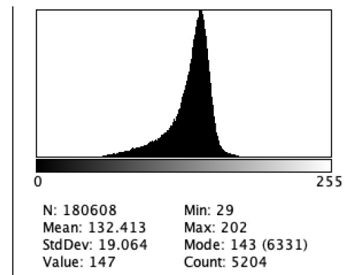
bluechannel histogram
